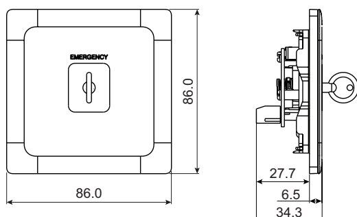
Panic Buttons with Key Reset
