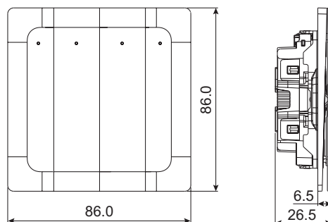
4G Switch
