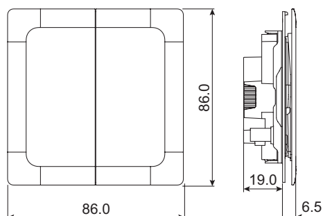
2G Intermediate Switch
