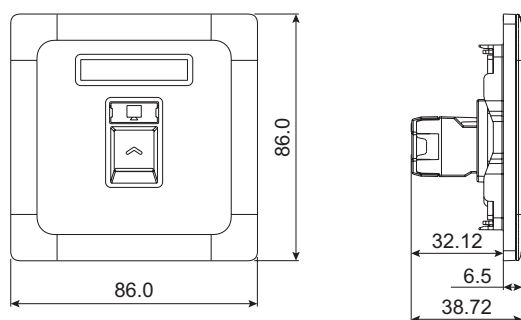
1G Cat. 6 RJ45 Shuttered Data Sockets
