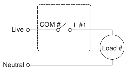
1-way Switch - 4 Gang
