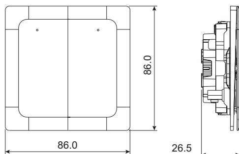
Switches with DND, PCU Symbol
