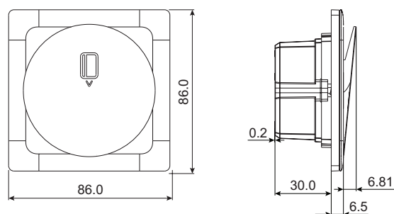
1G Electronic Key Card Switches
