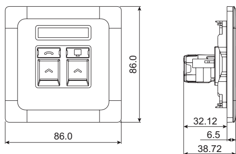
2G Cat. 6 RJ45 Shuttered Data Sockets (Telephone + Data)
