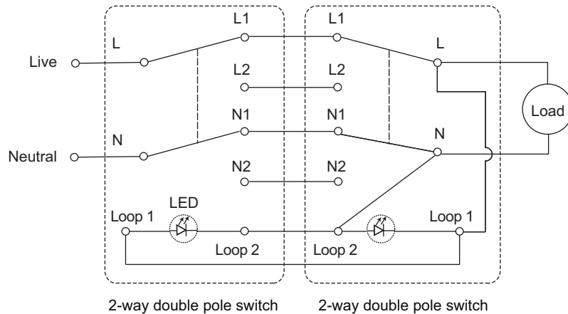
2-way Double Pole Switch
