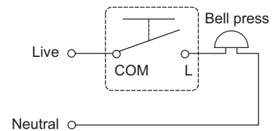
Bell Switch
