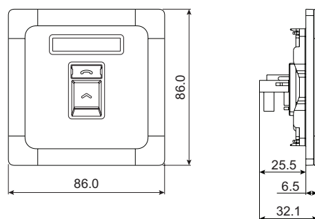
1G Shuttered Telephone Sockets
