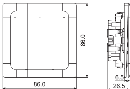
3G Switch
