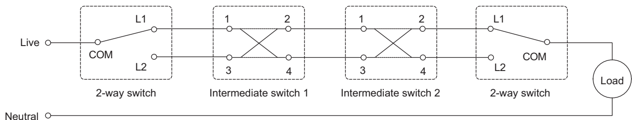
Intermediate Switch
