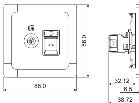
2G Cat. 6 RJ45 Shuttered Data Sockets (TV + Data)
