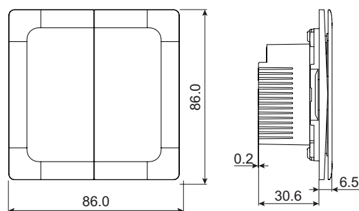
2G Universal Push Button Dimmers
