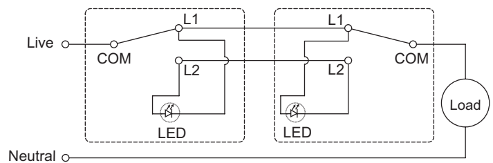
2-way Switch with LED Indicator
