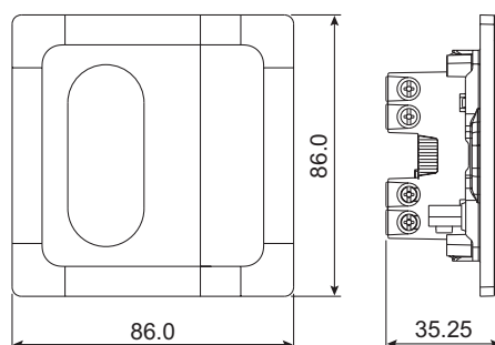
Bell Switches with DND, PCU Indicator
