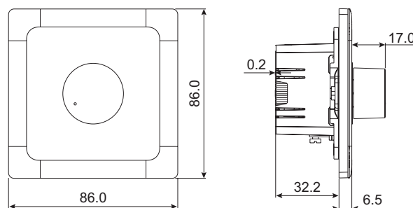
1G Fan Control Units with Rotary Knob
