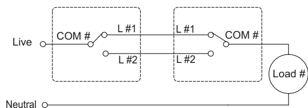
2-way Switch - 4 Gang
