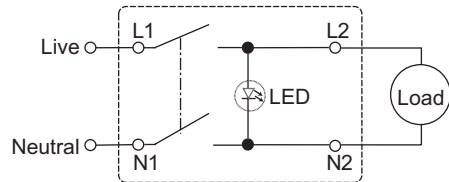
1-way Double Pole Switch
