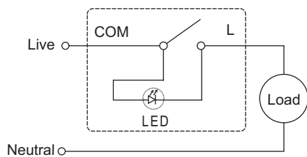
1-way Switch with LED Indicator
