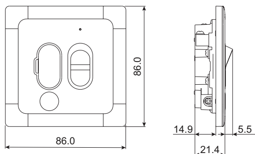
Double Pole 1G, Fuse Connection Units with LED Indicator – 13 A
