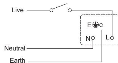
Switched Socket
